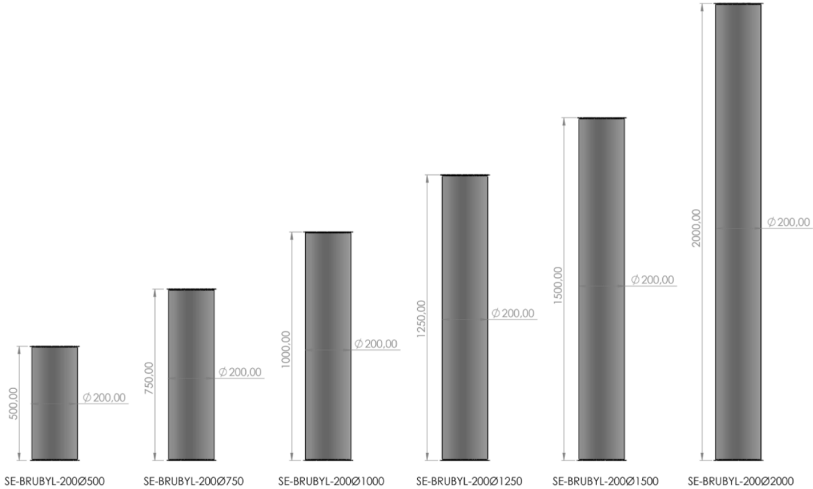
Flour & Grain Flow Pipes – Painted
