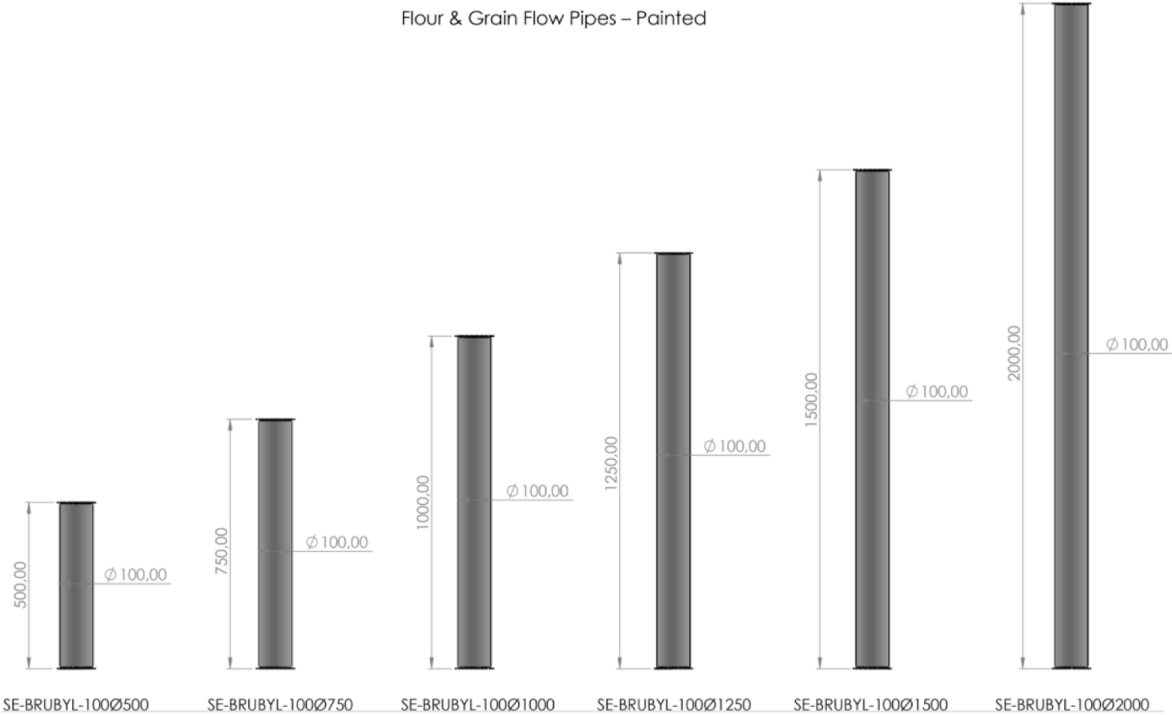
Flour & Grain Flow Pipes – Painted
