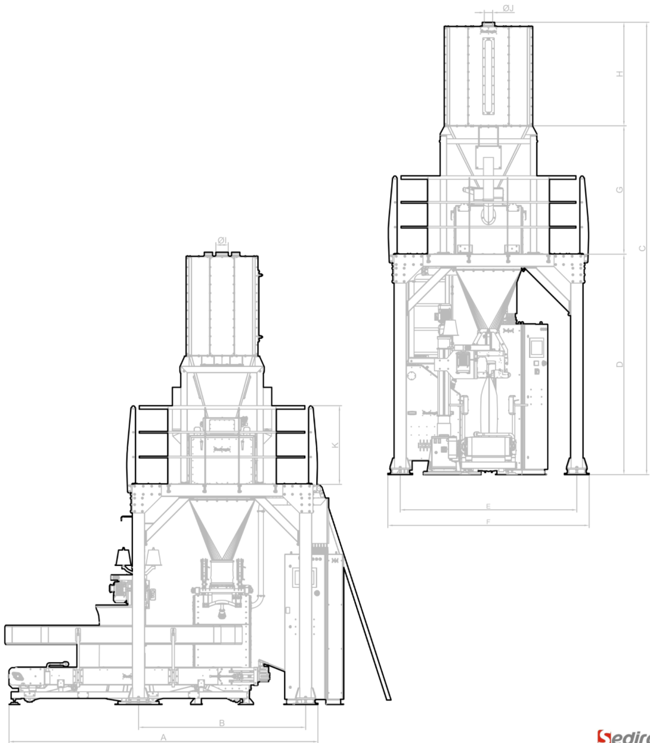
SE-PRD Granular Product Packing Machine 25/50 Kg (Single Spout)
